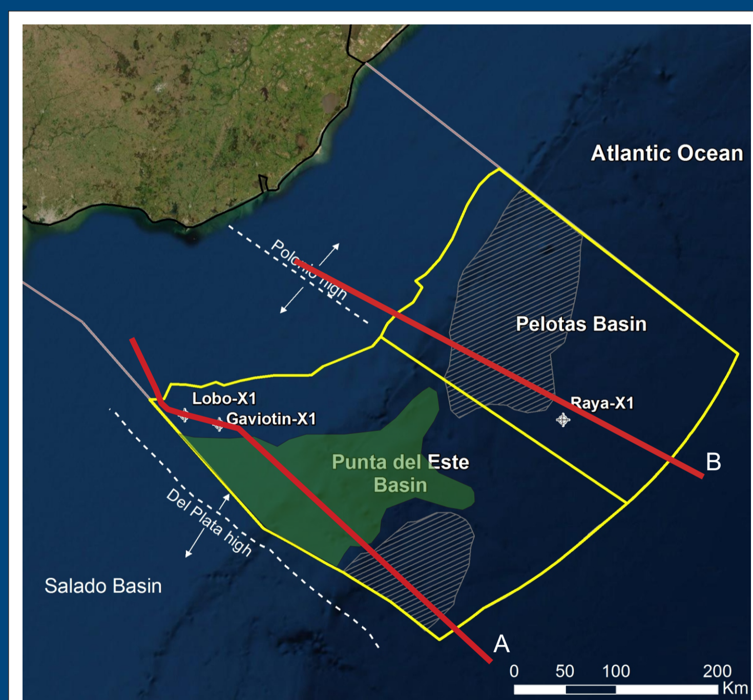
Synrift source rock
