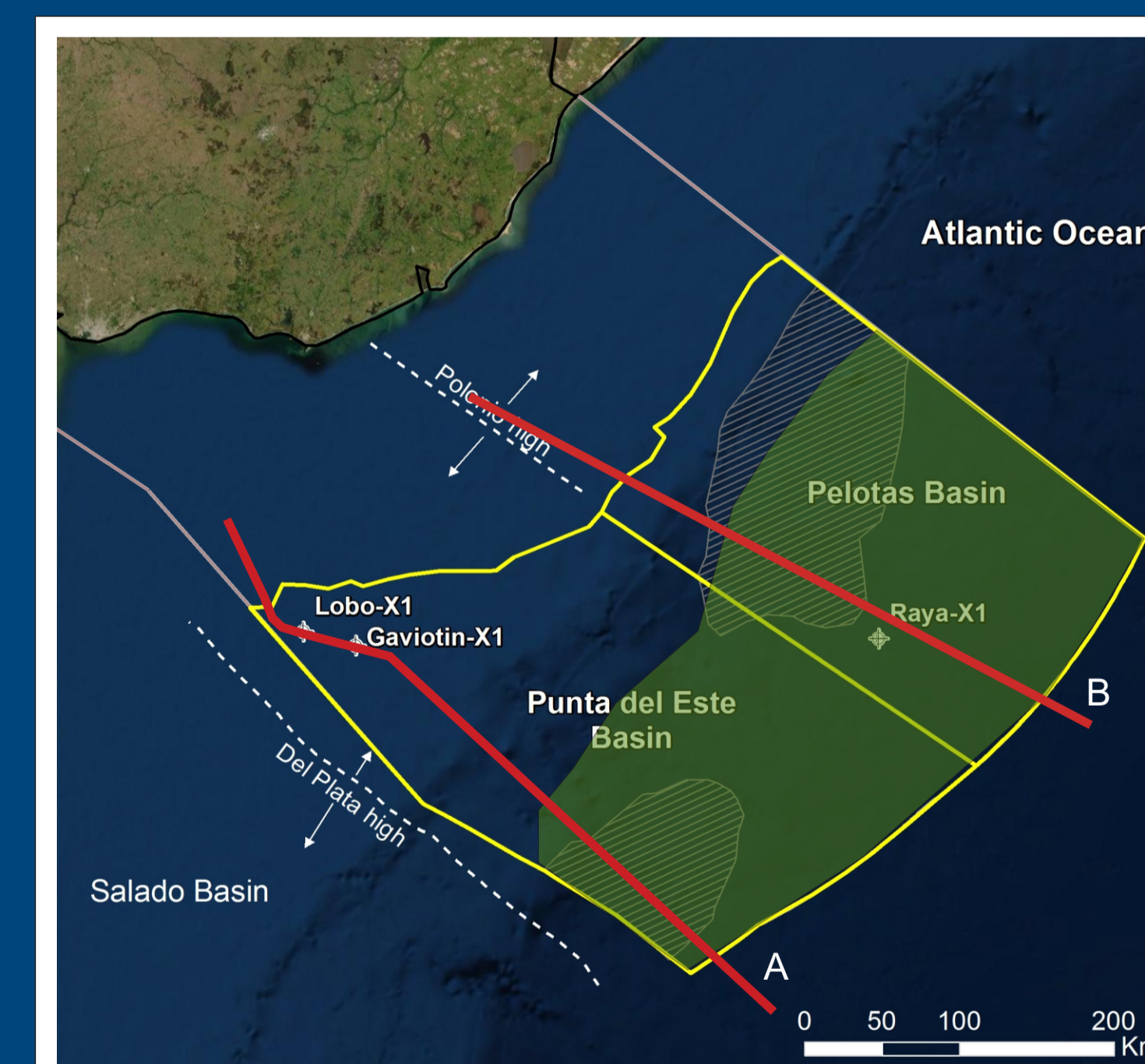
C-T source rock
