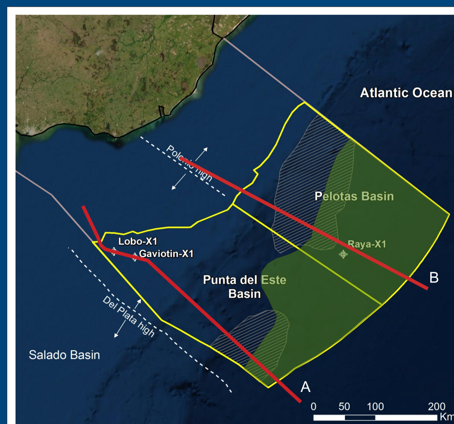
Aptian source rock
