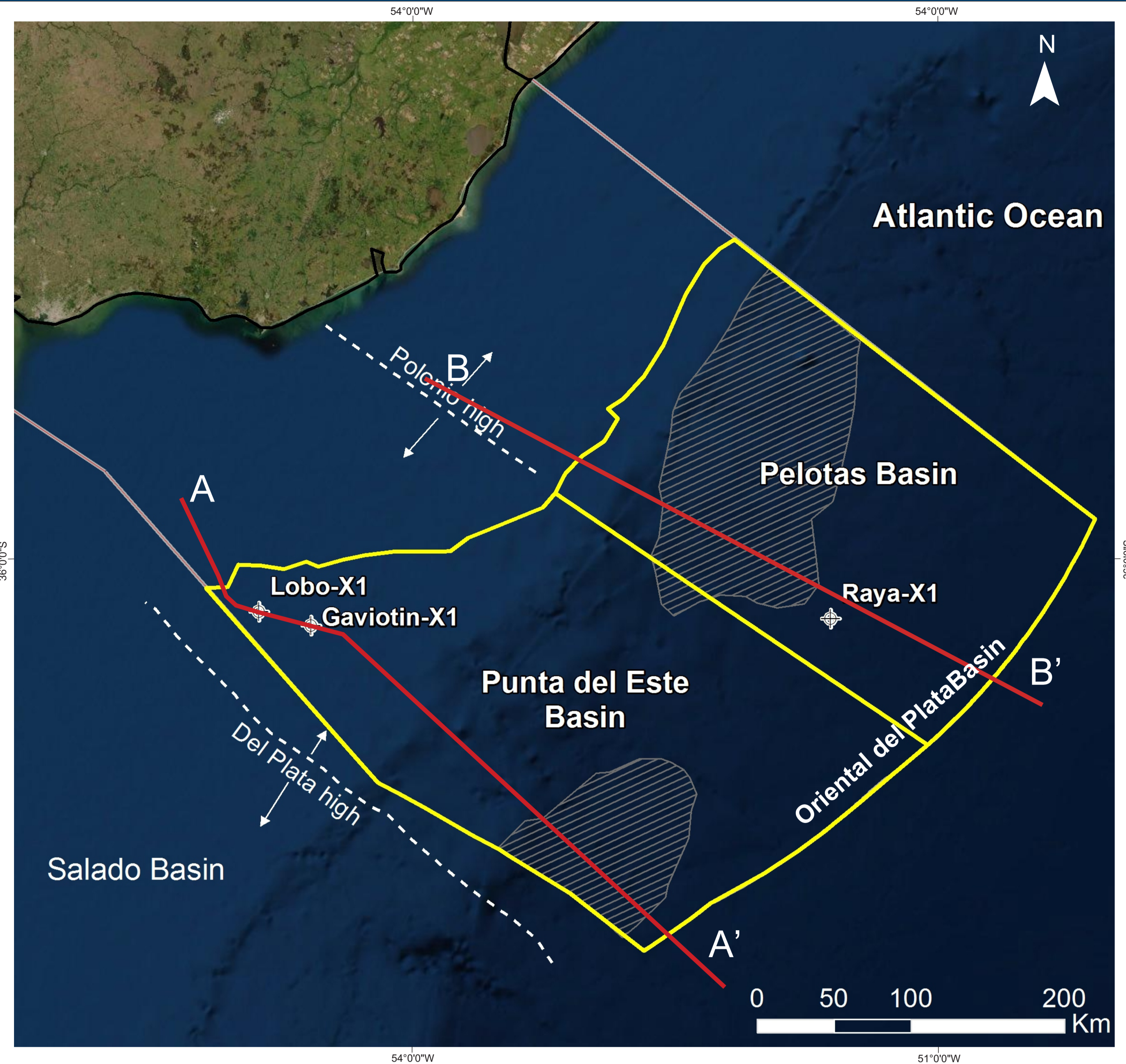
Offshore basins of Uruguay
