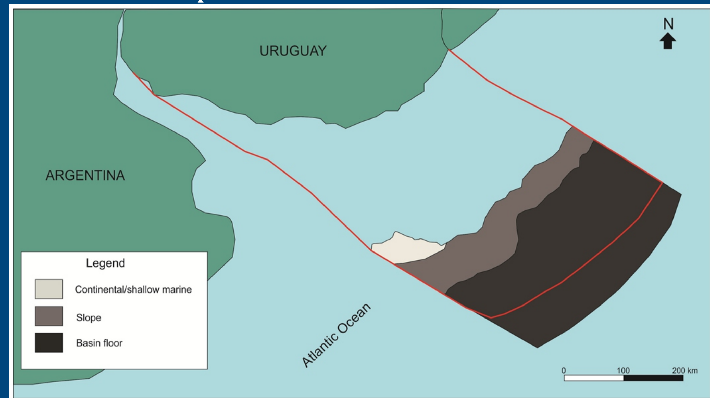
Aptian source rock distribution
